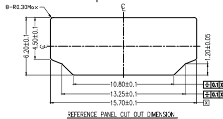
REFERENCE PANEL CUT OUT DIMENSION
