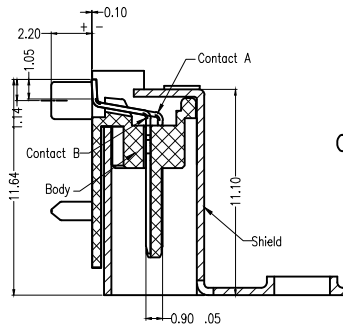
SECT:A-A
